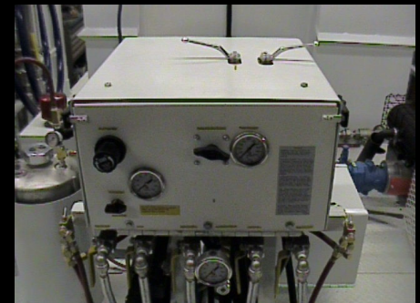
Center-mounted control console can be accessed from either operator station.
